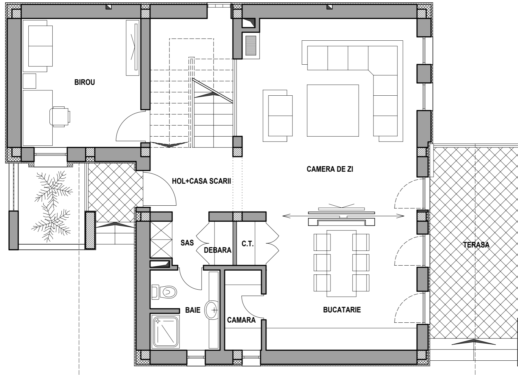
PLAN PARTER
